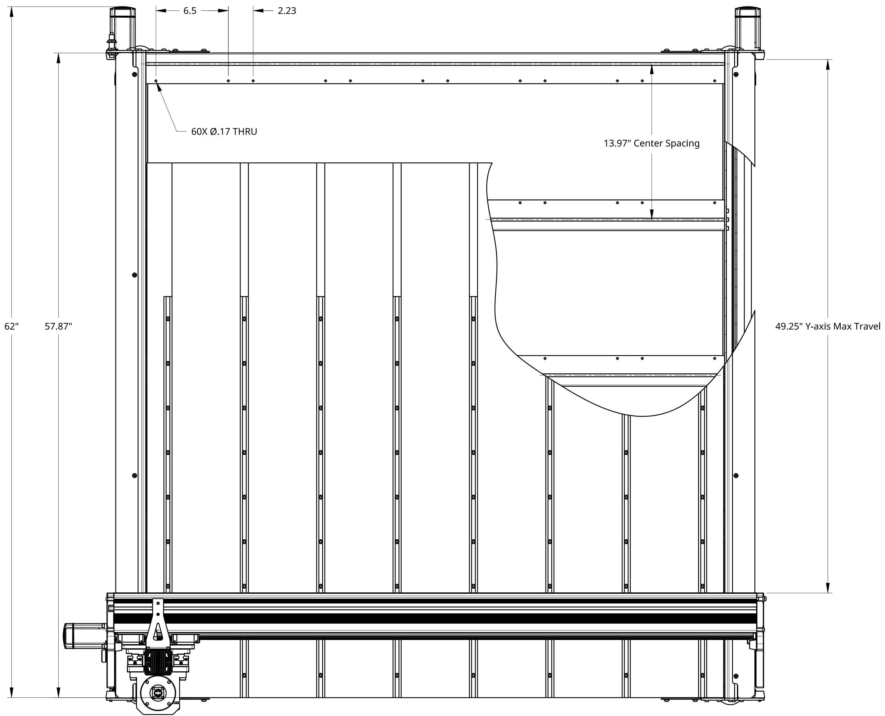
TOP VIEW
