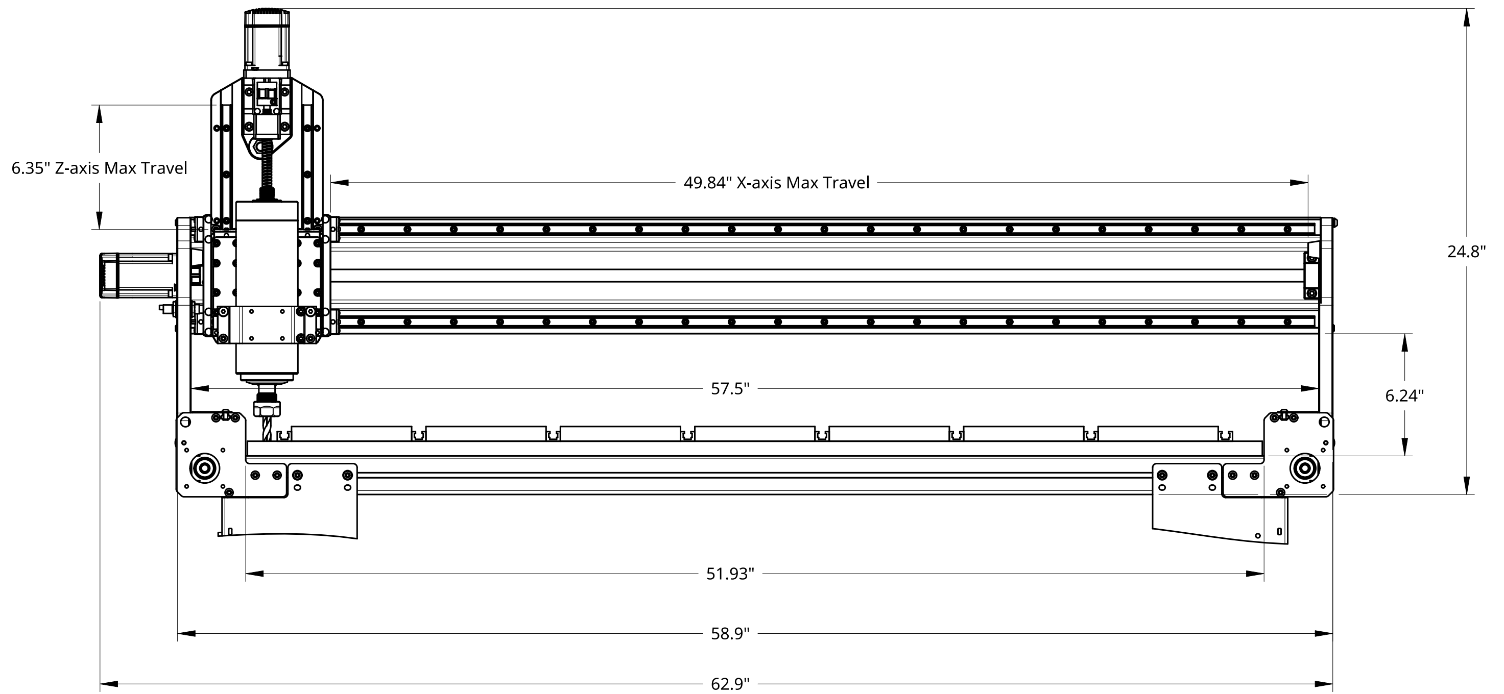
FRONT VIEW
